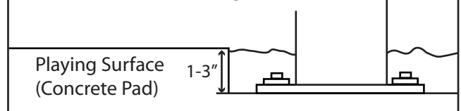
Figure 4: Pole Placement
