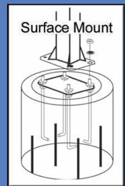
Heavy-duty anchor installation system for surface mounting.
